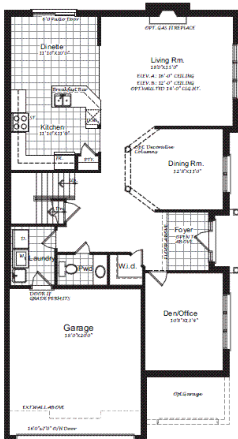
Main Floor
