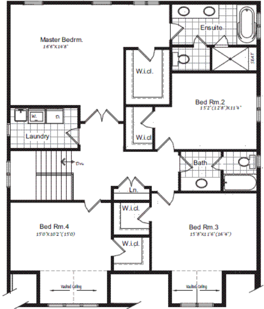
Second Floor
