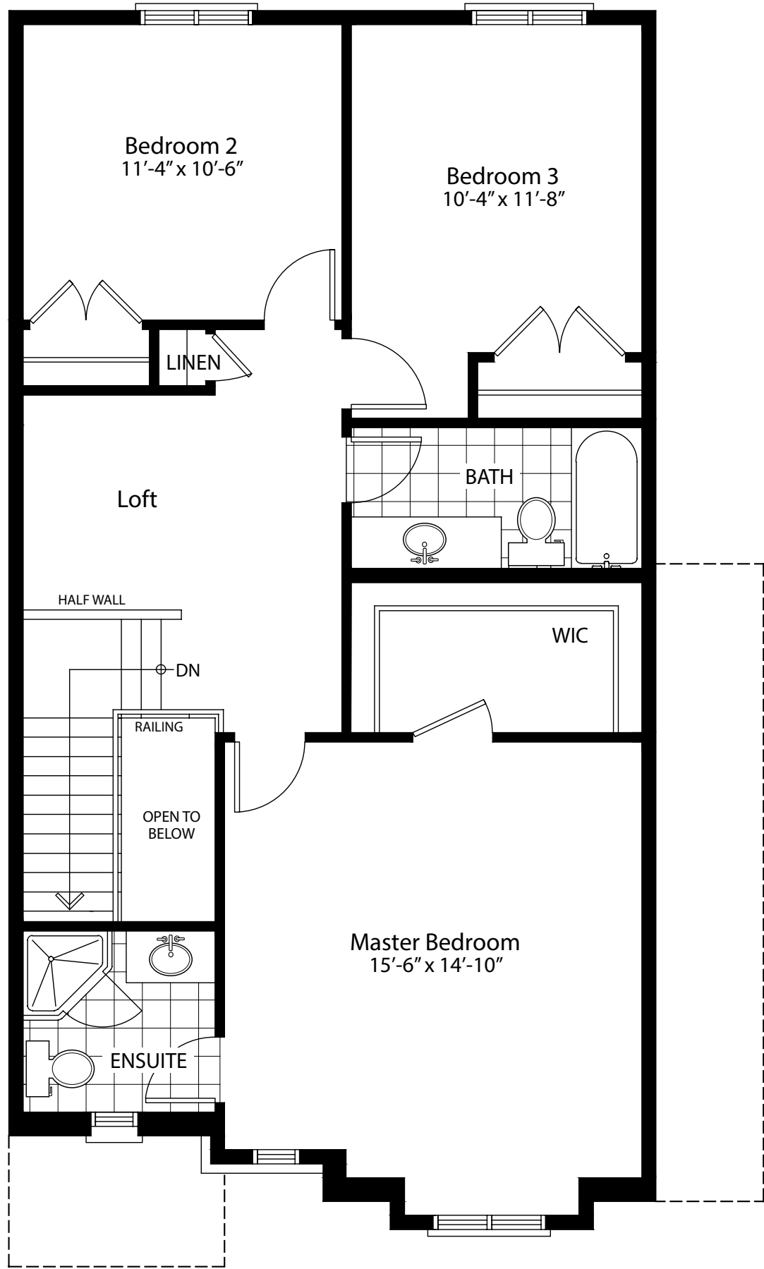
Second Floor
