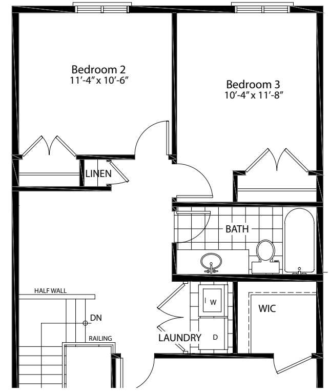
Second Floor • Opt. laundry
