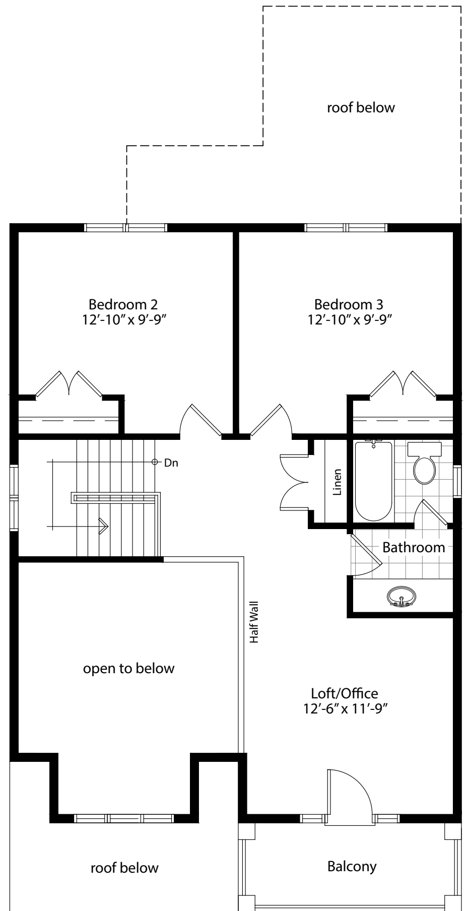
Second Floor
