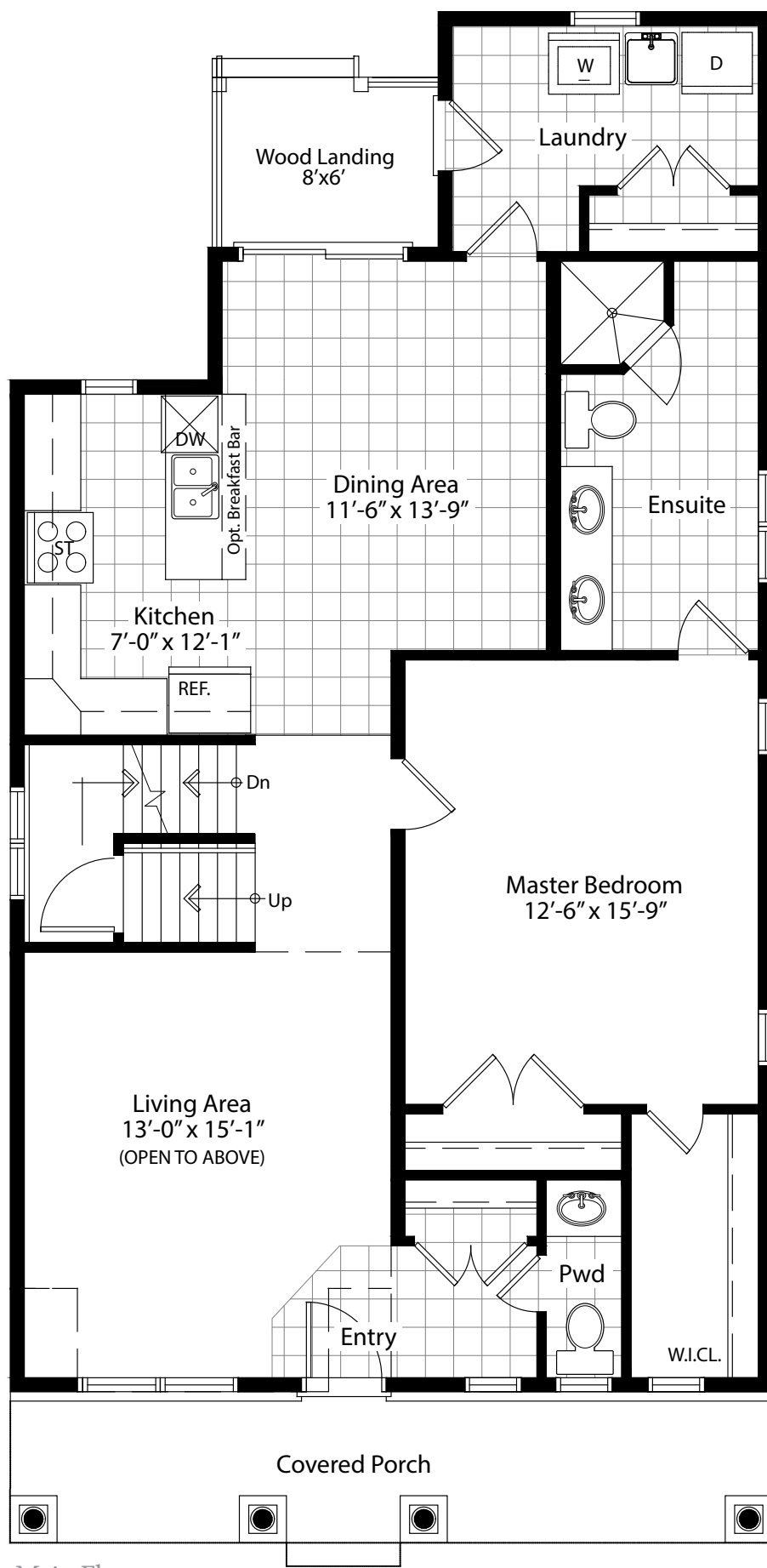
Main Floor
