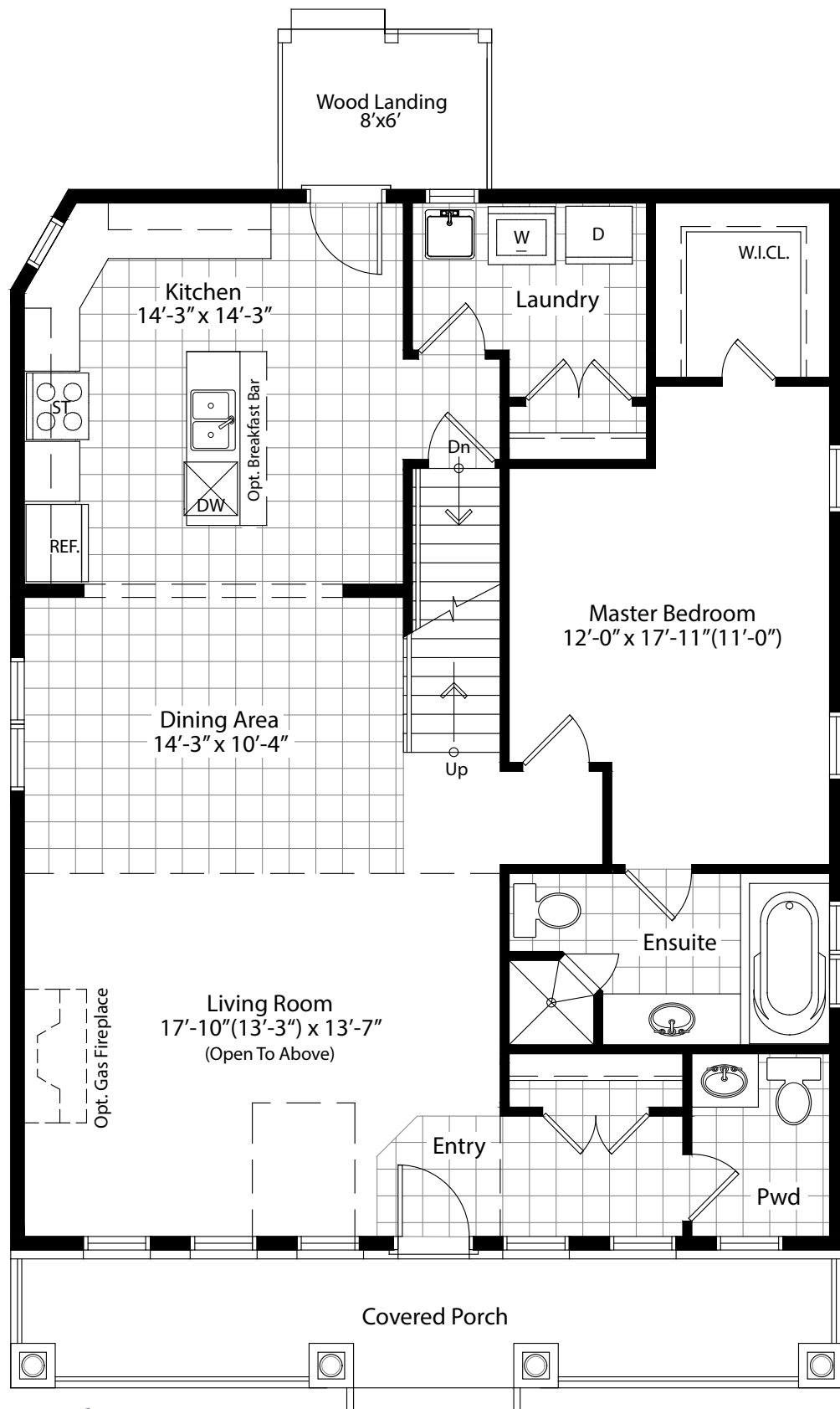
Main Floor
