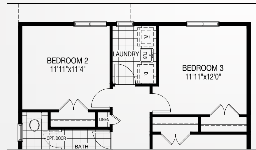
OPTION 2 SECOND FLOOR - W/LAUNDRY
