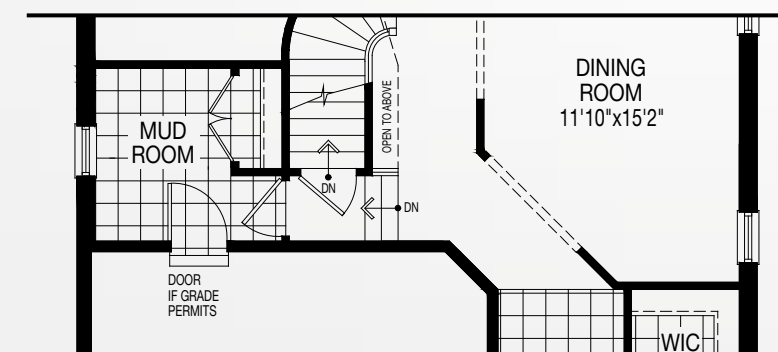
OPTION 2 GROUND FLOOR - W/MUD ROOM
