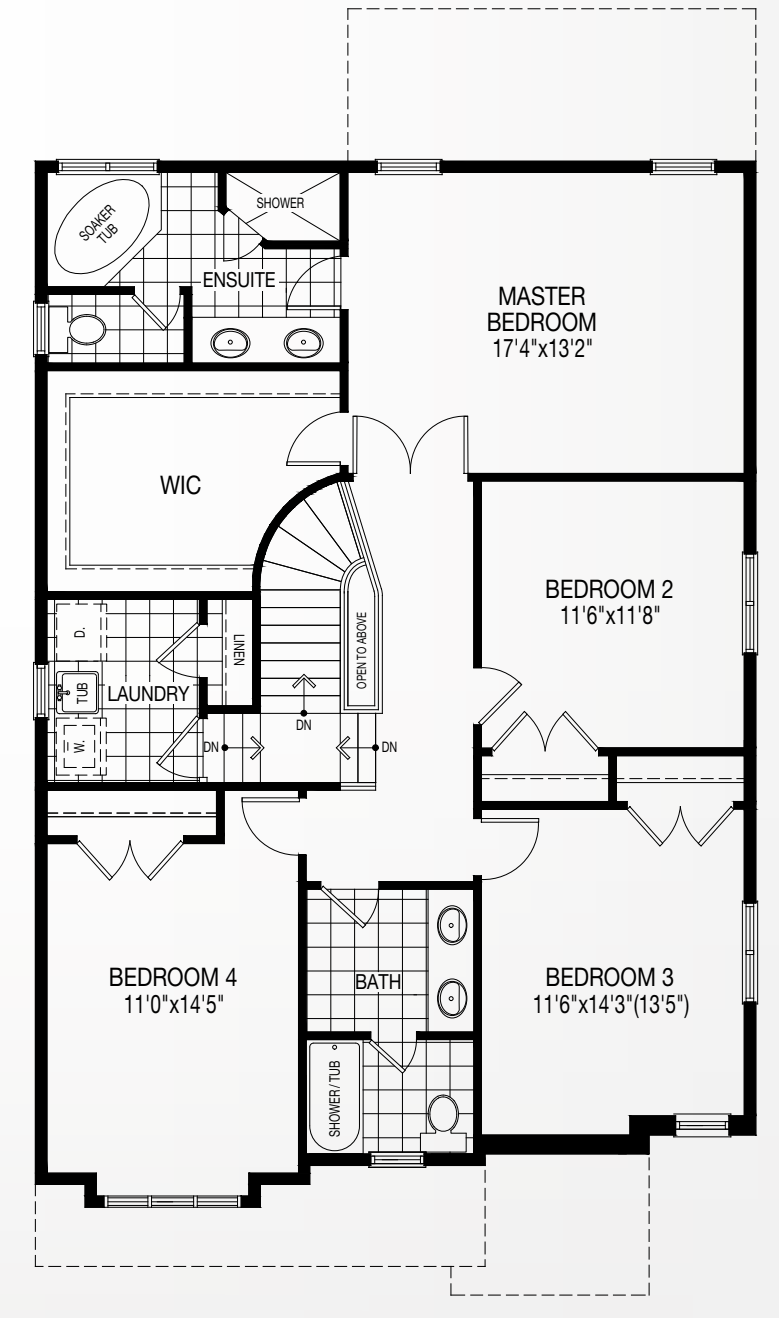
OPTION 2 SECOND FLOOR - W/LAUNDRY
